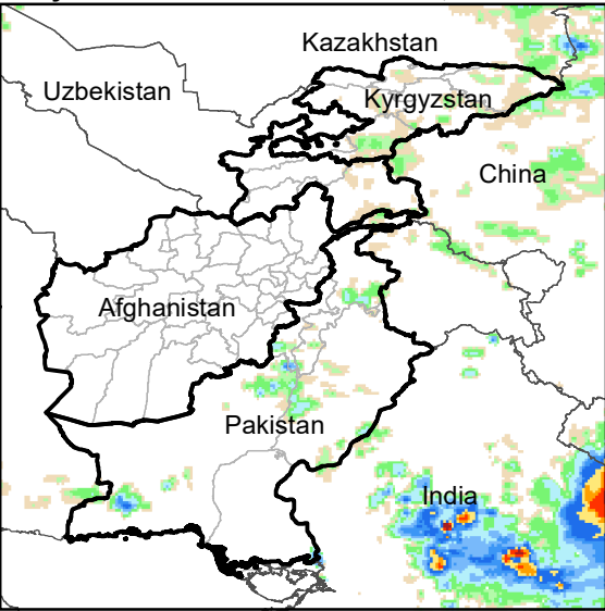
Daily Rainfall estimate for 17 Jul., 2007
