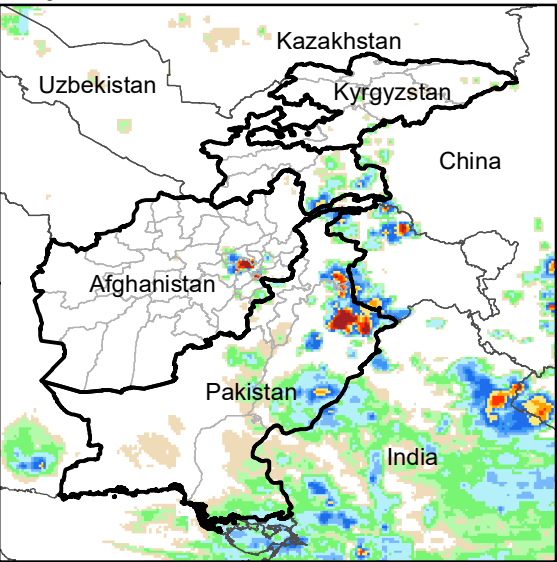
Daily Rainfall estimate for 2 Aug., 2007
