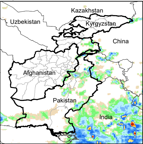
Daily Rainfall estimate for 1 Aug., 2007
