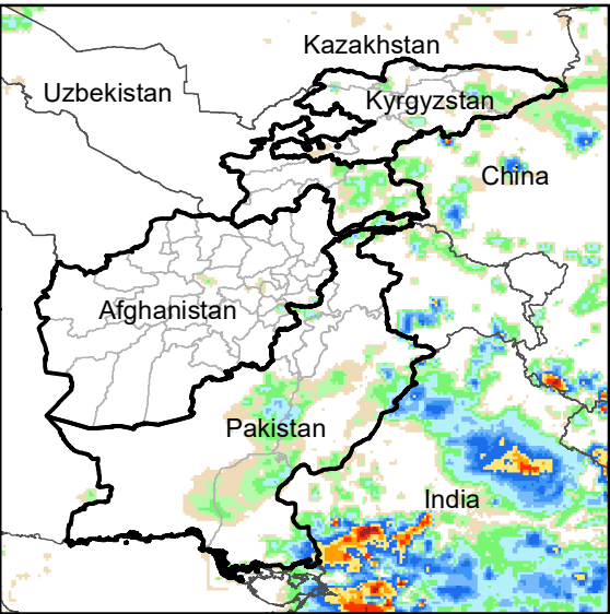
Daily Rainfall estimate for 31 Jul., 2007
