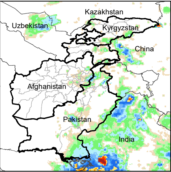
Daily Rainfall estimate for 5 Aug., 2007
