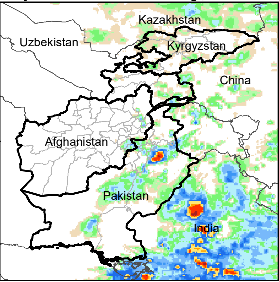
Daily Rainfall estimate for 3 Aug., 2007
