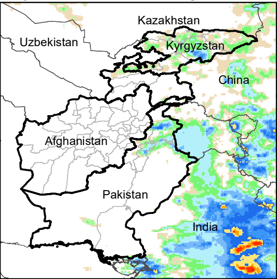
Daily Rainfall estimate for 4 Aug., 2007
