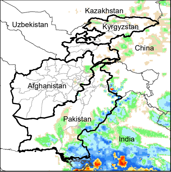
Daily Rainfall estimate for 7 Aug., 2007
