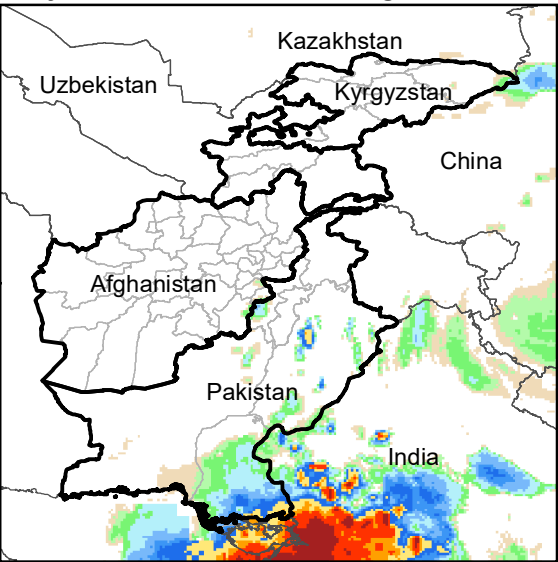
Daily Rainfall estimate for 11 Aug., 2007
