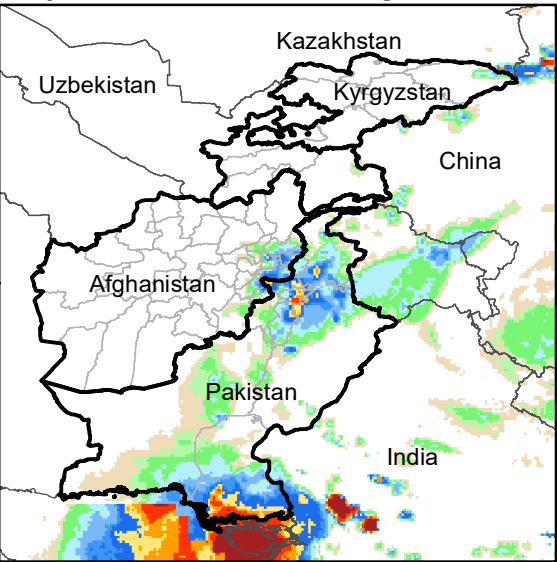
Daily Rainfall estimate for 12 Aug., 2007
