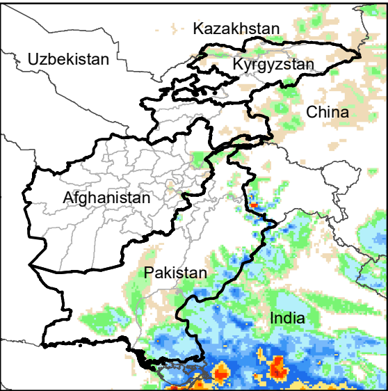
Daily Rainfall estimate for 10 Aug., 2007
