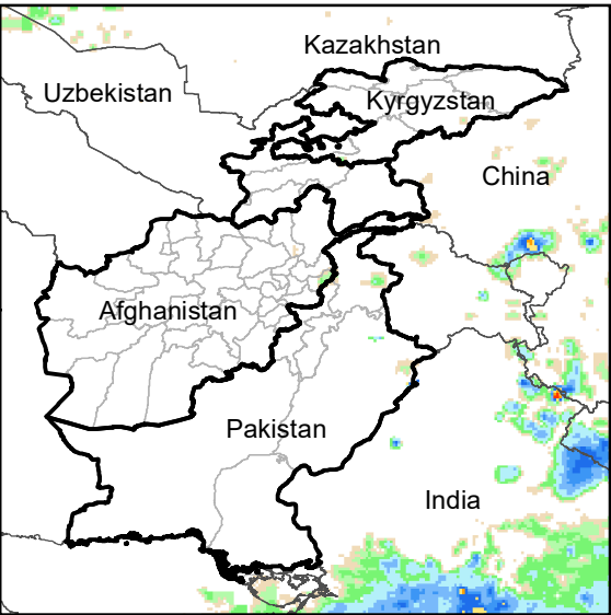
Daily Rainfall estimate for 22 Sep., 2007
