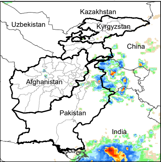
Daily Rainfall estimate for 23 Sep., 2007
