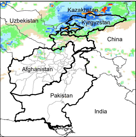
Daily Rainfall estimate for 26 Nov., 2007
