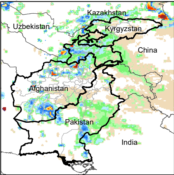
Daily Rainfall estimate for 13 Dec., 2007
