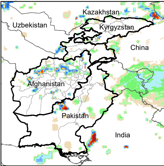
Daily Rainfall estimate for 14 Dec., 2007
