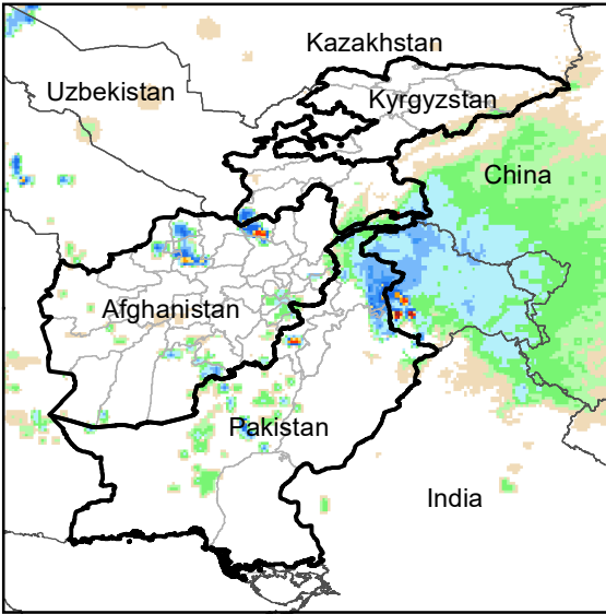
Daily Rainfall estimate for 18 Jan., 2008
