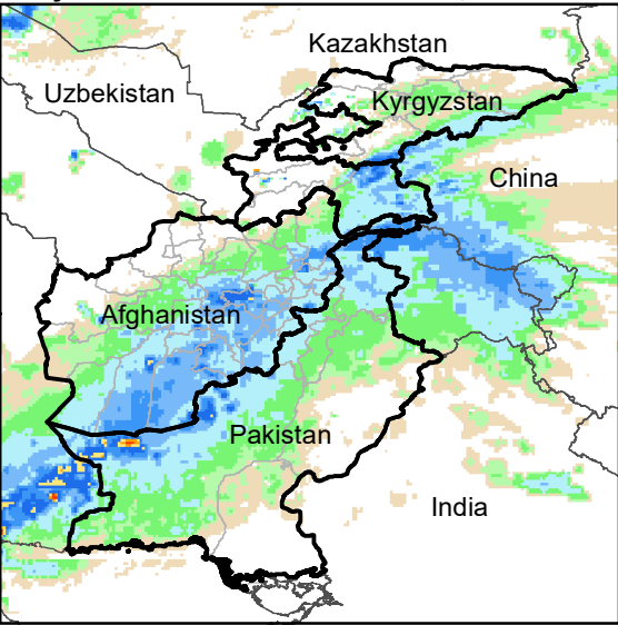
Daily Rainfall estimate for 16 Jan., 2008
