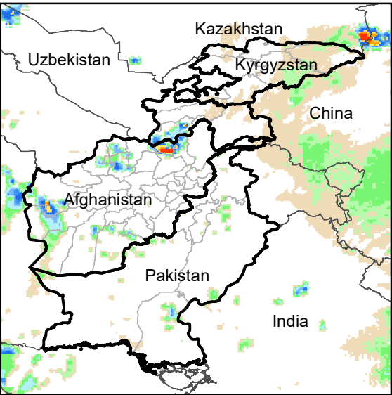
Daily Rainfall estimate for 26 Jan., 2008
