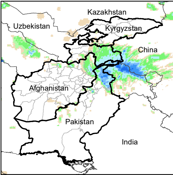
Daily Rainfall estimate for 4 Feb., 2008
