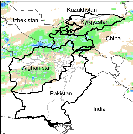
Daily Rainfall estimate for 19 Feb., 2008
