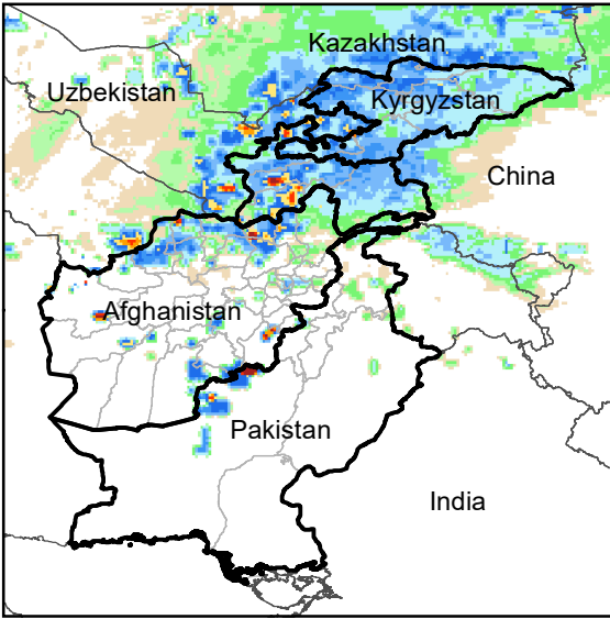
Daily Rainfall estimate for 21 Feb., 2008
