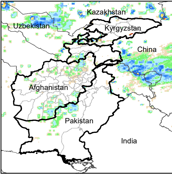
Daily Rainfall estimate for 24 Feb., 2008
