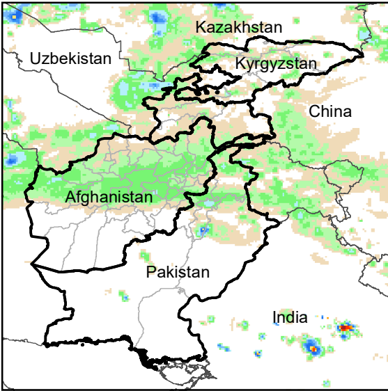
Daily Rainfall estimate for 13 Apr., 2008
