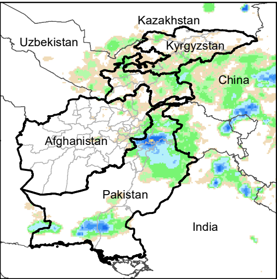
Daily Rainfall estimate for 28 May., 2008
