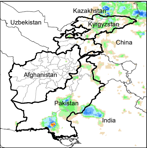
Daily Rainfall estimate for 5 Jun., 2008
