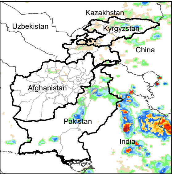
Daily Rainfall estimate for 10 Jun., 2008
