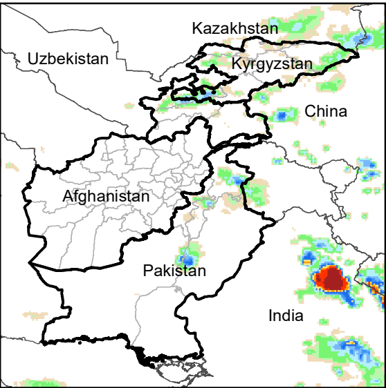
Daily Rainfall estimate for 9 Jun., 2008
