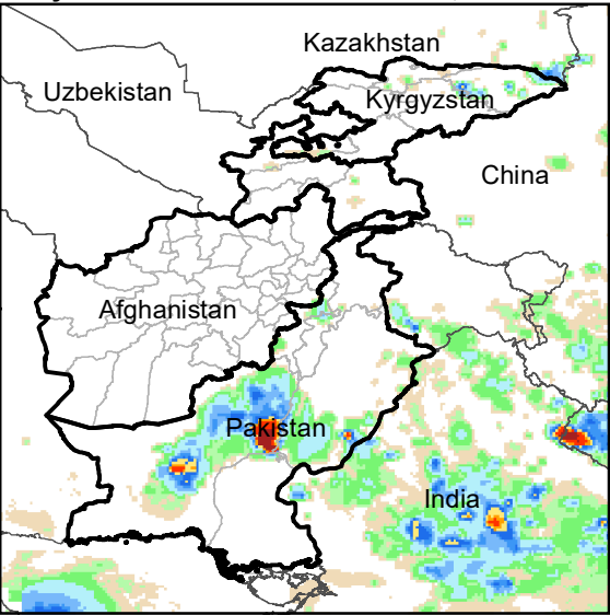
Daily Rainfall estimate for 11 Jun., 2008
