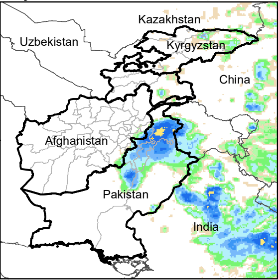
Daily Rainfall estimate for 16 Jun., 2008
