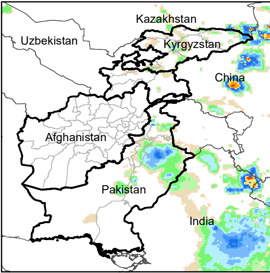
Daily Rainfall estimate for 18 Jun., 2008
