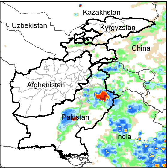
Daily Rainfall estimate for 2 Jul., 2008
