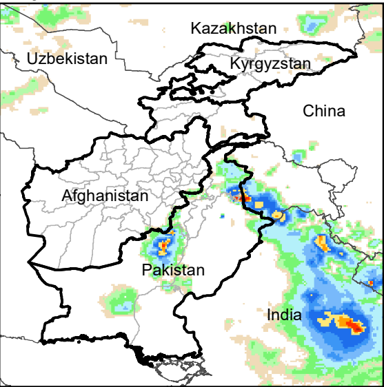
Daily Rainfall estimate for 8 Jul., 2008
