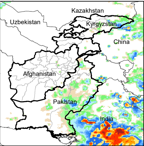
Daily Rainfall estimate for 13 Jul., 2008
