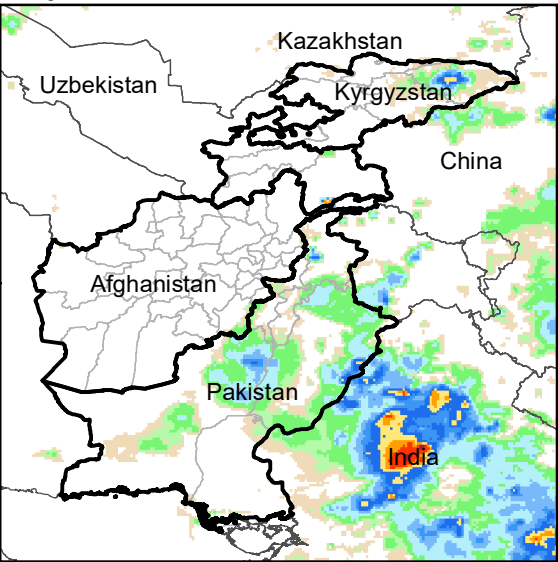
Daily Rainfall estimate for 12 Jul., 2008
