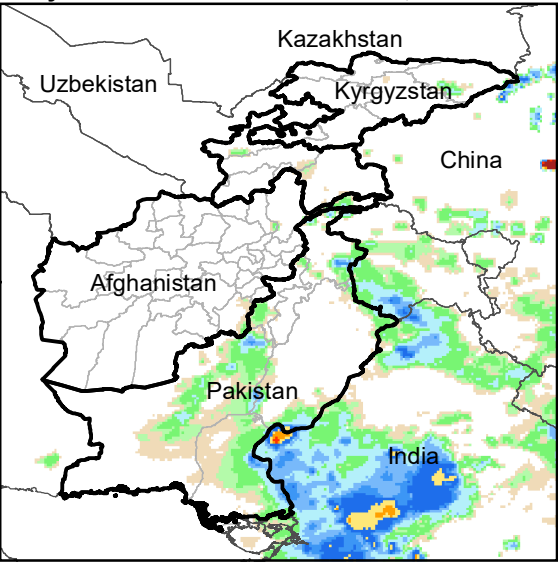
Daily Rainfall estimate for 11 Jul., 2008
