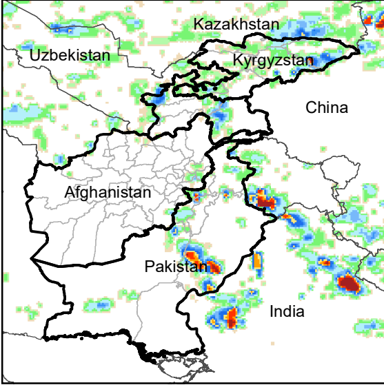
Daily Rainfall estimate for 17 Jul., 2008
