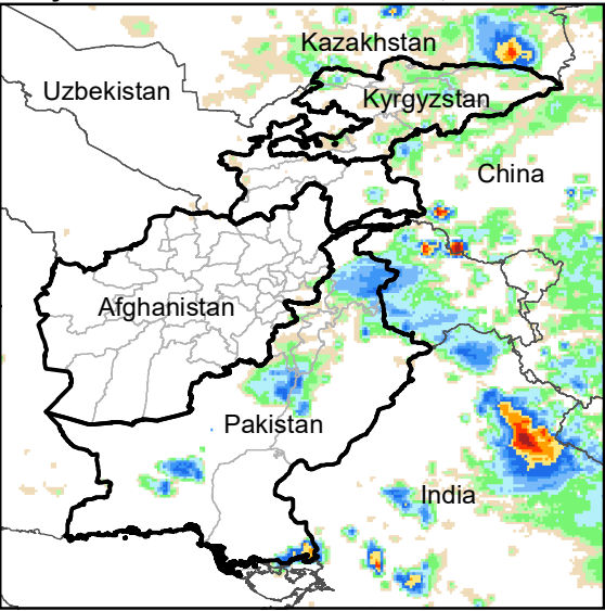
Daily Rainfall estimate for 18 Jul., 2008
