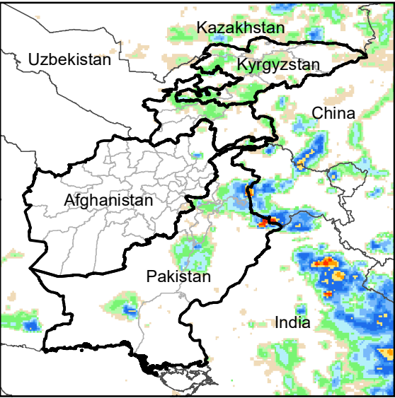
Daily Rainfall estimate for 19 Jul., 2008
