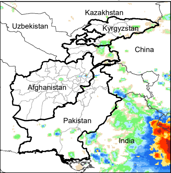
Daily Rainfall estimate for 10 Aug., 2008
