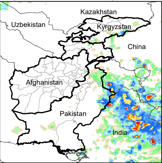
Daily Rainfall estimate for 11 Aug., 2008
