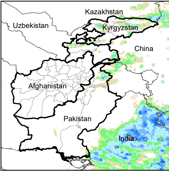
Daily Rainfall estimate for 26 Aug., 2008
