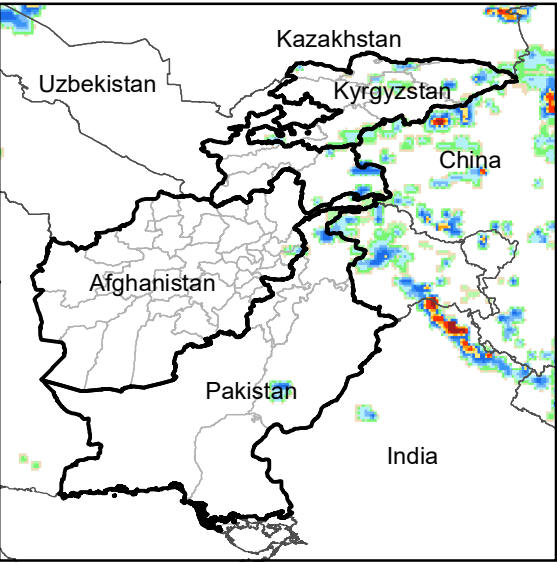
Daily Rainfall estimate for 24 Sep., 2008
