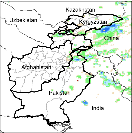
Daily Rainfall estimate for 26 Sep., 2008
