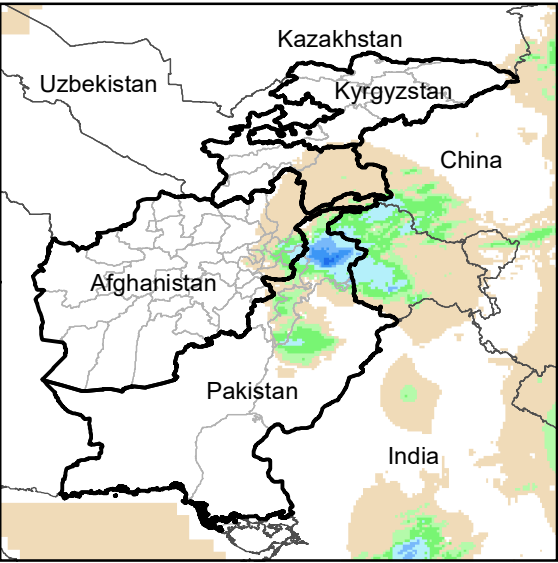
Daily Rainfall estimate for 7 Oct., 2008
