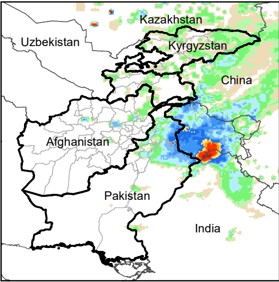
Daily Rainfall estimate for 15 Oct., 2008
