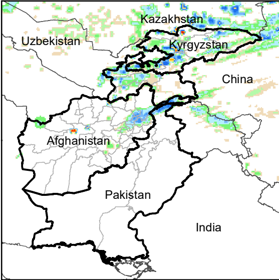
Daily Rainfall estimate for 12 Nov., 2008
