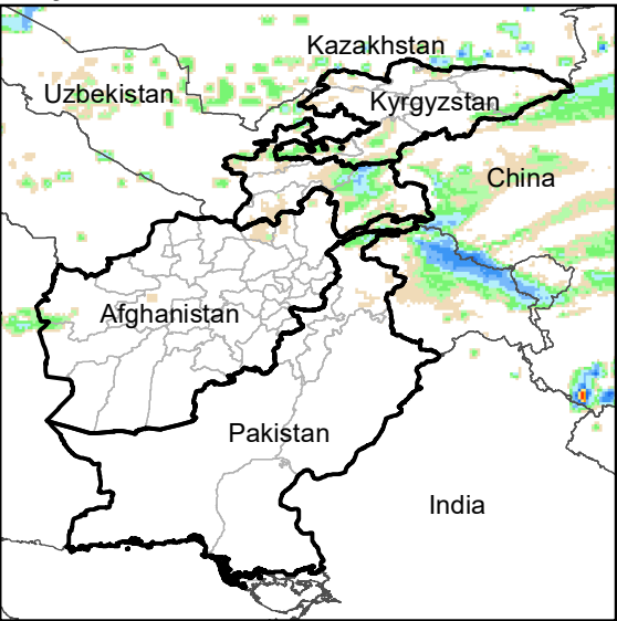
Daily Rainfall estimate for 14 Nov., 2008
