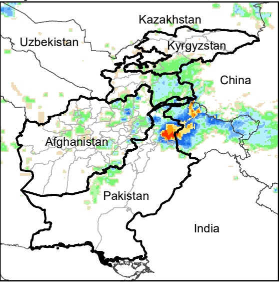
Daily Rainfall estimate for 13 Nov., 2008
