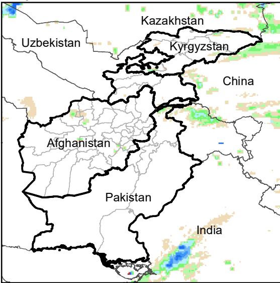
Daily Rainfall estimate for 4 Dec., 2008
