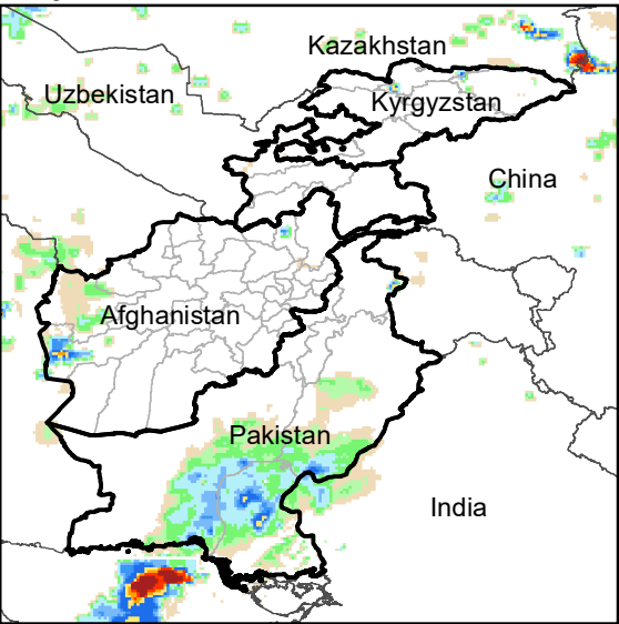
Daily Rainfall estimate for 9 Dec., 2008
