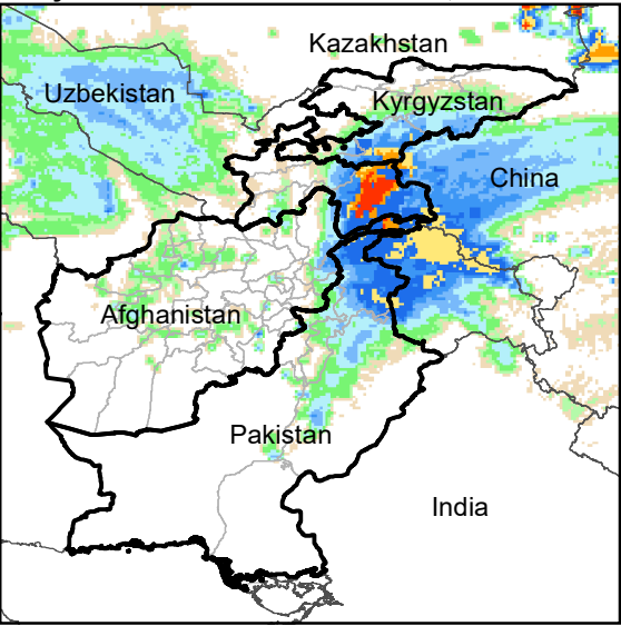
Daily Rainfall estimate for 8 Dec., 2008
