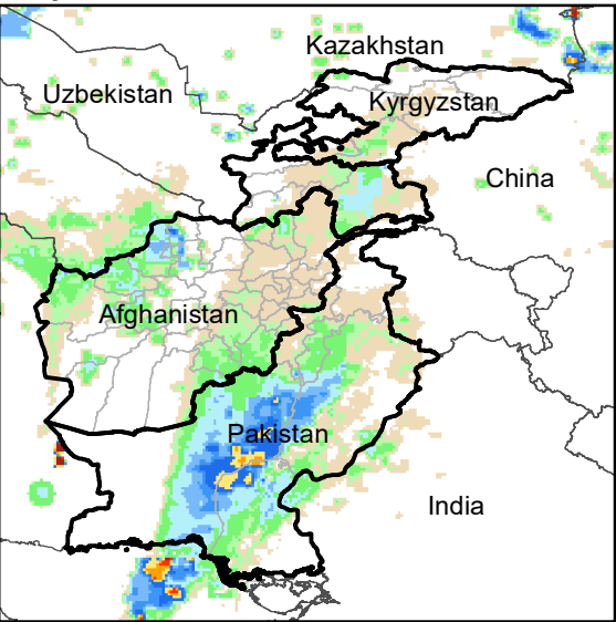
Daily Rainfall estimate for 10 Dec., 2008
