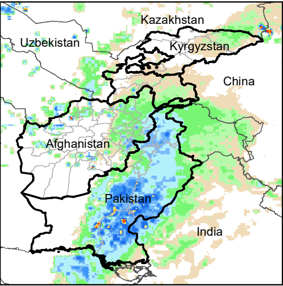
Daily Rainfall estimate for 19 Dec., 2008
