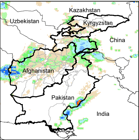
Daily Rainfall estimate for 18 Dec., 2008
