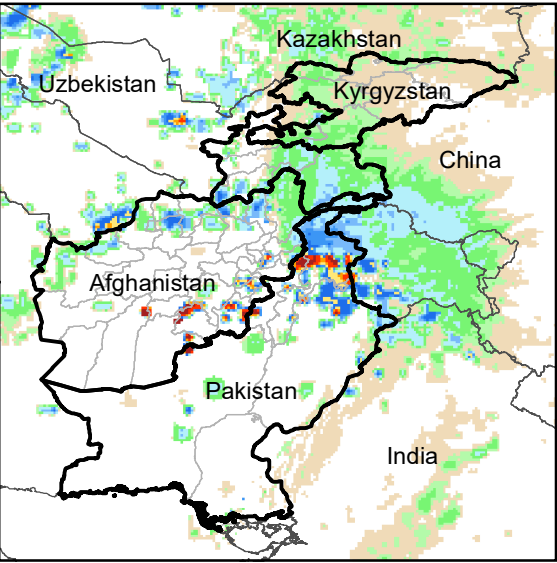
Daily Rainfall estimate for 20 Dec., 2008
