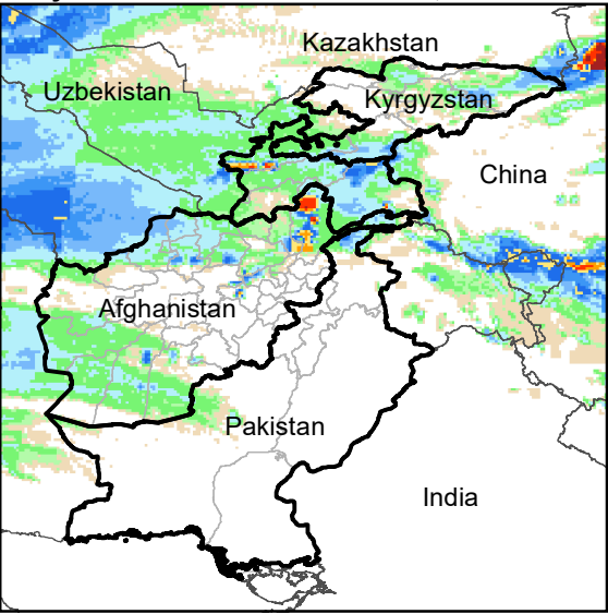
Daily Rainfall estimate for 1 Jan., 2009
