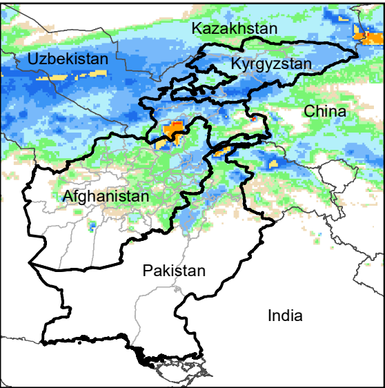
Daily Rainfall estimate for 5 Feb., 2009
