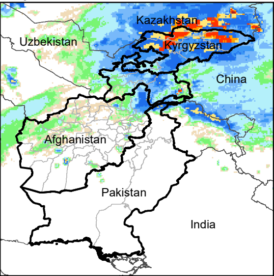
Daily Rainfall estimate for 6 Feb., 2009
