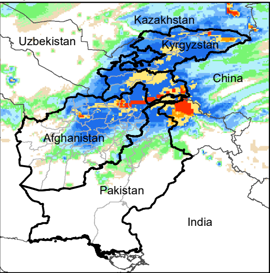
Daily Rainfall estimate for 7 Feb., 2009
