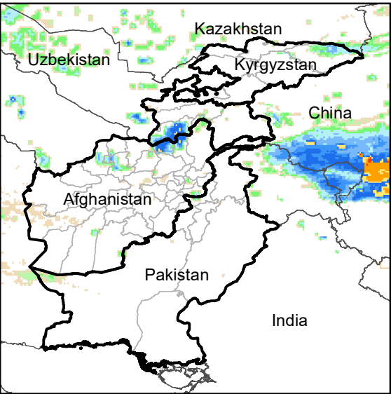
Daily Rainfall estimate for 2 Mar., 2009
