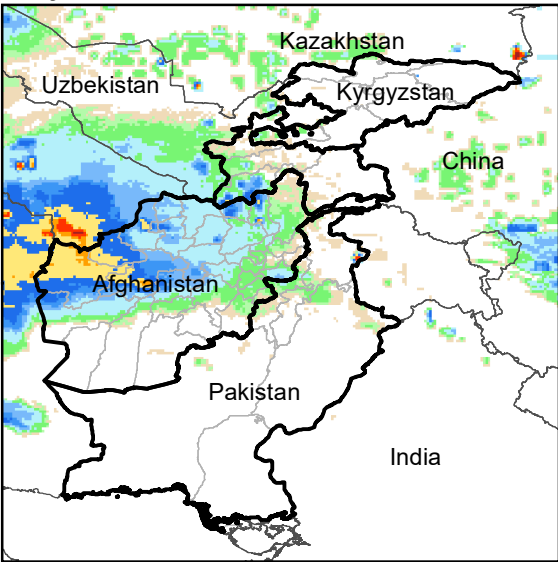
Daily Rainfall estimate for 3 Mar., 2009
