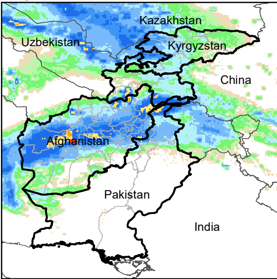
Daily Rainfall estimate for 4 Mar., 2009
