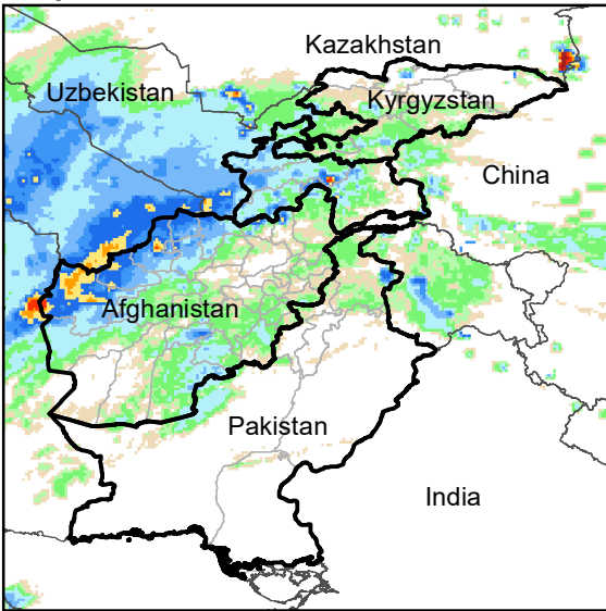
Daily Rainfall estimate for 5 Mar., 2009
