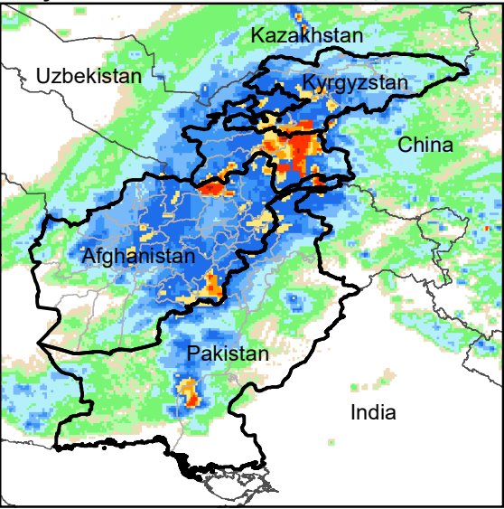
Daily Rainfall estimate for 23 Mar., 2009
