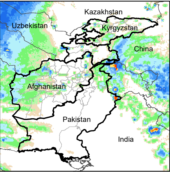
Daily Rainfall estimate for 25 Mar., 2009
