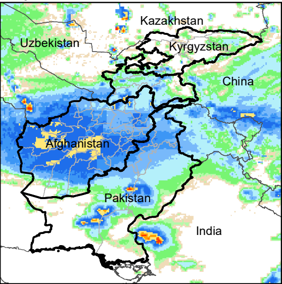
Daily Rainfall estimate for 24 Mar., 2009
