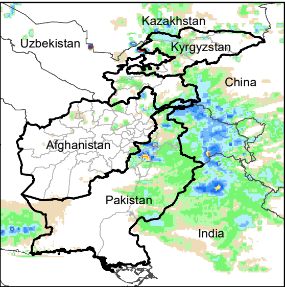
Daily Rainfall estimate for 30 Mar., 2009
