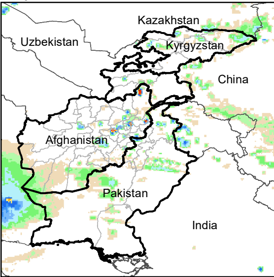
Daily Rainfall estimate for 2 Apr., 2009
