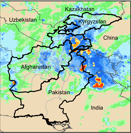
Daily Rainfall estimate for 6 Apr., 2009
