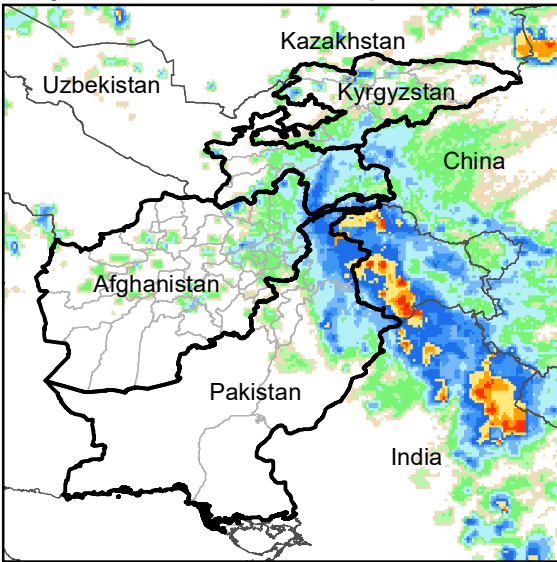
Daily Rainfall estimate for 11 Apr., 2009
