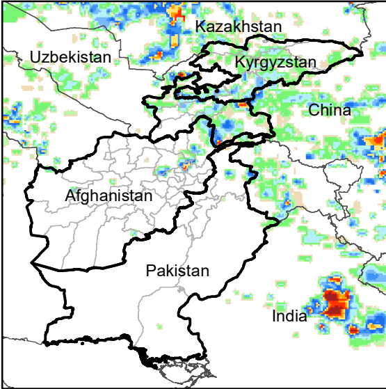
Daily Rainfall estimate for 13 May., 2009
