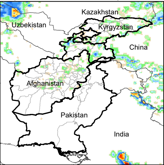
Daily Rainfall estimate for 16 May., 2009
