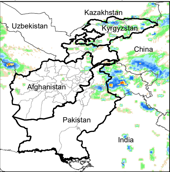
Daily Rainfall estimate for 28 May., 2009
