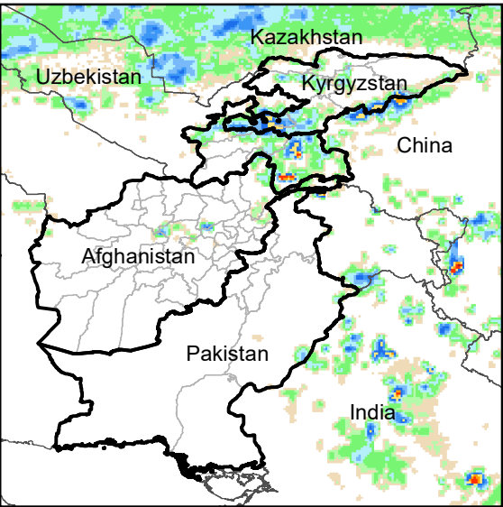
Daily Rainfall estimate for 26 May., 2009
