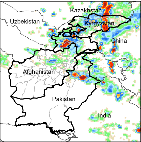
Daily Rainfall estimate for 27 May., 2009
