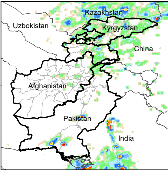
Daily Rainfall estimate for 26 Jun., 2009
