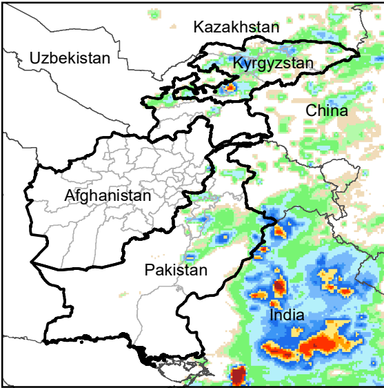
Daily Rainfall estimate for 13 Jul., 2009
